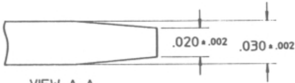
VIEW A-A (ENLARGED)
